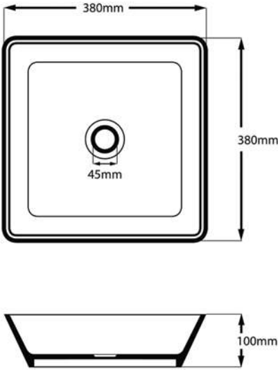
Quadrato Basin | Weight: 5kg Size: 380mm x 380mm Water Capacity: 9 litres
