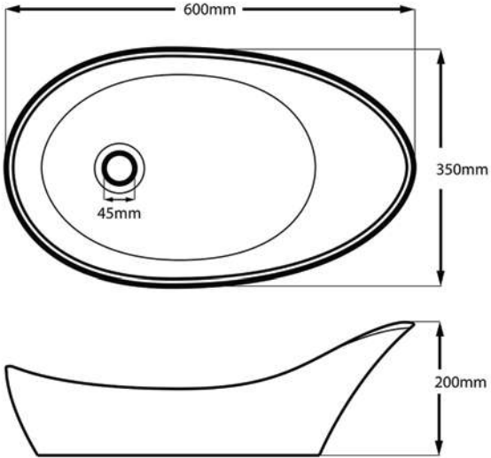
Classic Basin | Weight: 8kg Size: 600mm x 350mm Water Capacity: 8 litres
