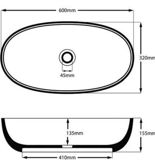
Pebble Basin | Weight: 10kg Size: 600mm x 320mm Water Capacity: 14 litres
