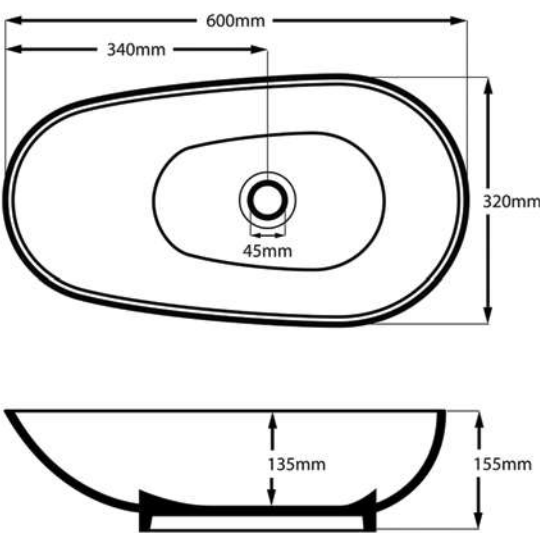
Cocoon Basin | Weight: 7kg Size: 600mm x 320mm Water Capacity: 13 litres
