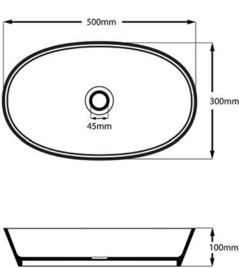
Petite Basin | Weight: 5kg Size: 500mm x 300mm Water Capacity: 8 litres
