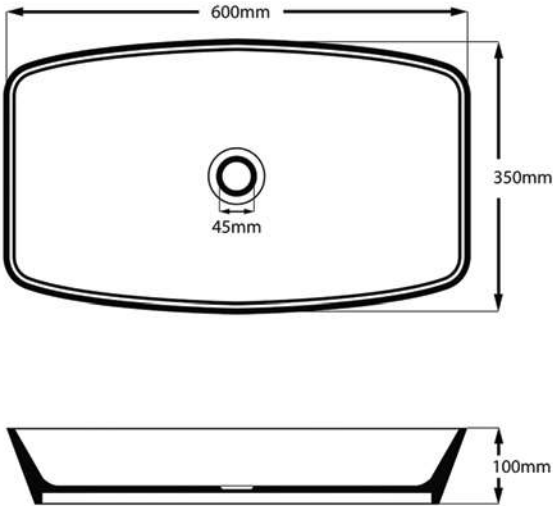
Geo Basin | Weight: 6kg Size: 600mm x 350mm Water Capacity: 11 litres
