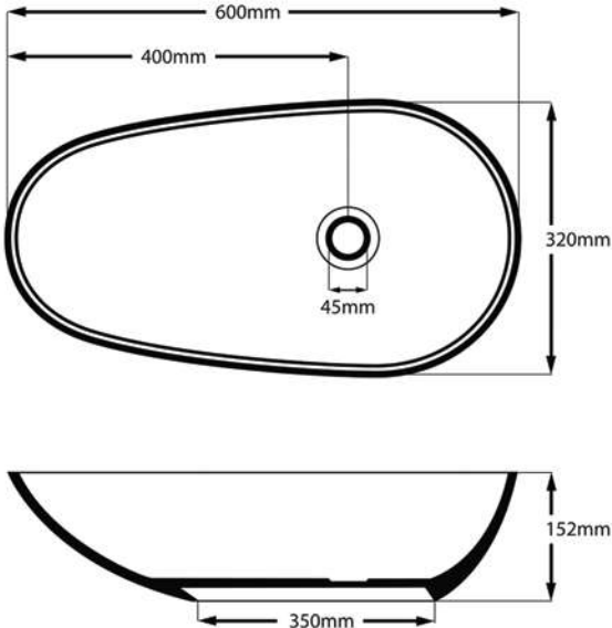
Ovale Basin | Weight: 8.5kg Size: 600mm x 320mm Water Capacity: 14 litres
