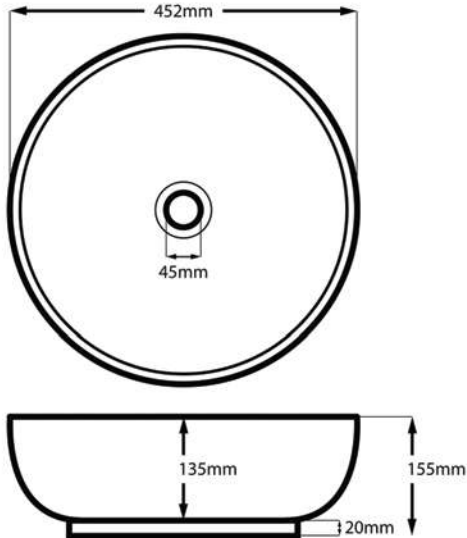
Oasis Basin | Weight: 8.5kg Size: 452mm x 452mm Water Capacity: 14 litres
