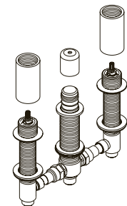
Deck-Mount Bath Faucet Valve
