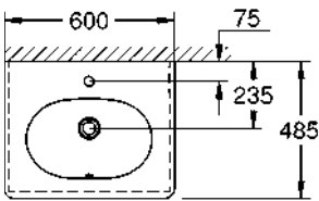
39 565 00H Wall hung basin, 60 cm
