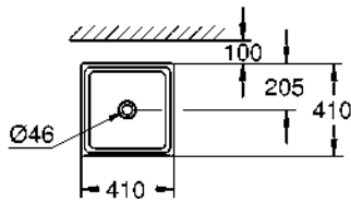
39 482 00H Vessel basin, 40 cm
