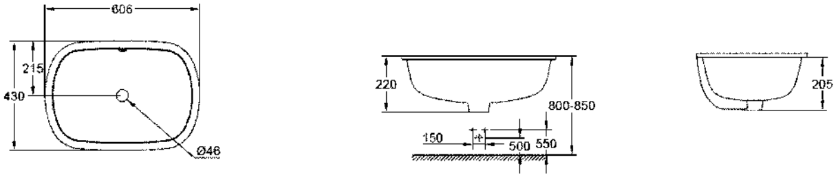
39 125 001 Under-counter basin, 60 cm
