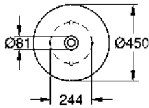
39 609 00H Vessel, 45 cm
