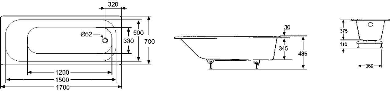
39 150 000 Bath tub - drop-in 170 x 70 cm
