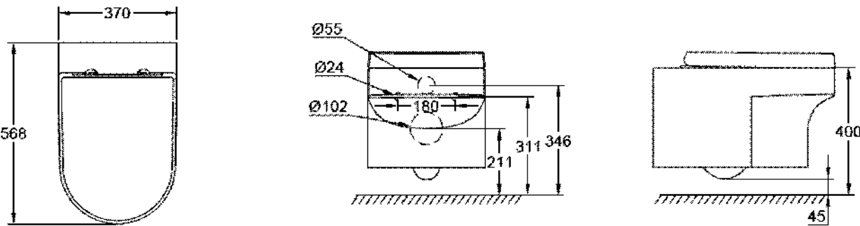
39 296 000 Wall hung WC
