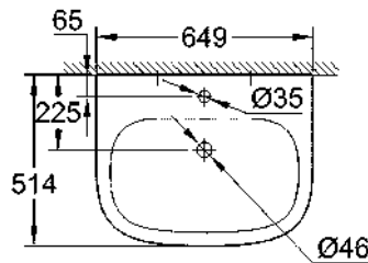
39 323 00H Wall hung basin, 65 cm
