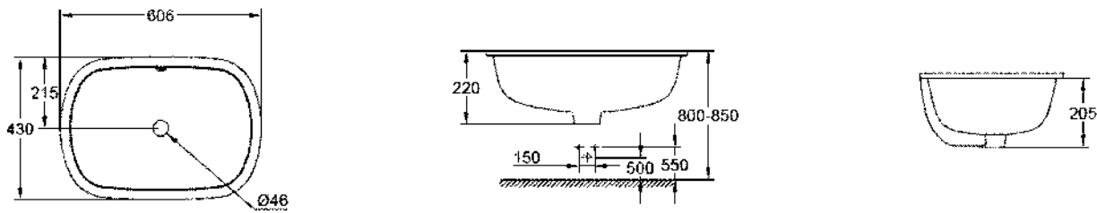
39 125 001 Under-counter basin, 60 cm
