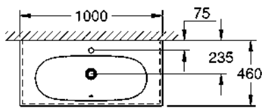
39 566 00H Vanity basin, 100 cm
