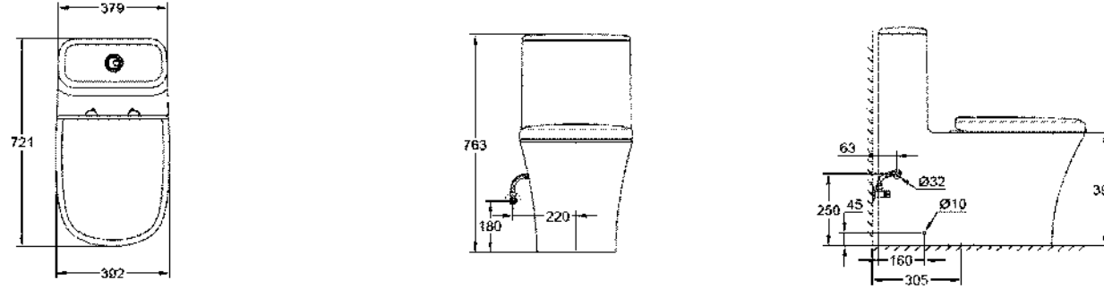
39 310 000 Floorstanding 1 PC WC
