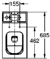
39 485 00H Floorstanding WC back to wall
