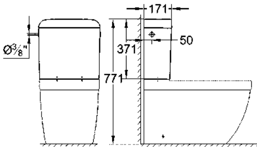
39 333 000 Cistern with side and back inlet
