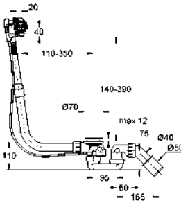
28 991 000 Talentofill inlet, waste & overflow valve
