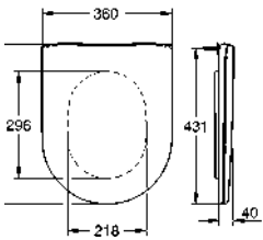
39 577 000 WC seat soft close
