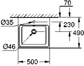
39 474 00H Wall hung basin, 50 cm
