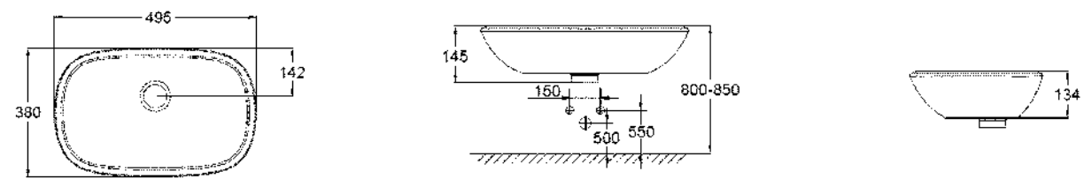
39 216 000 Vessel basin, 50 cm
