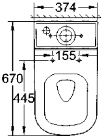
39 338 00H Floorstanding WC for closed coupled combination triple vortex, wash down, universal outlet, w/o cistern and seat
