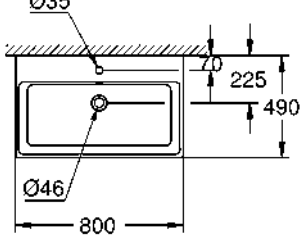
39 469 00H Wall hung basin, 80 cm
