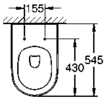
39 573 00H Floor standing WC back to wall
