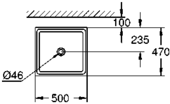
39 481 00H Vessel basin, 50 cm
