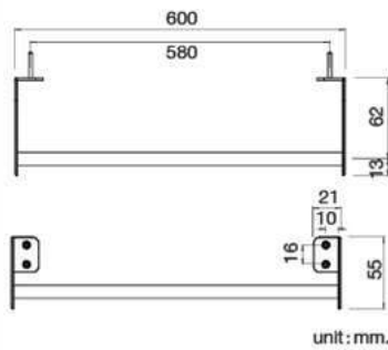
▲ FBVHY-G101AS Towel Bar Length 600 mm.
