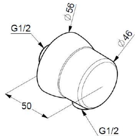
Dimensional drawing
